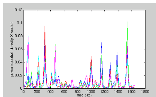
Fig. 3 Frequency Spectrum with 512 samples and 8.533 KHz sampling frequency
