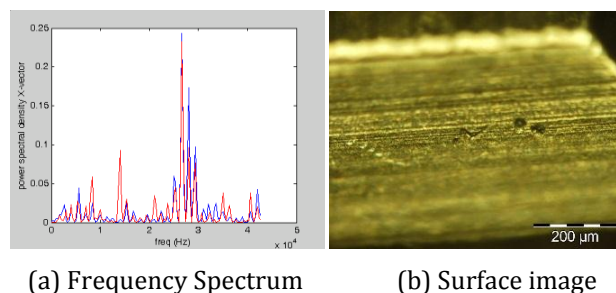
Fig.4 Frequency Spectrum and surface image after 1.5 \times 10^6 revolutions
