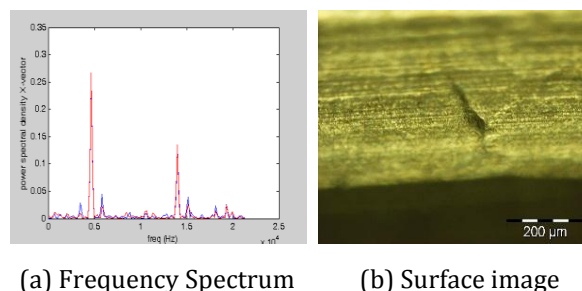
Fig. 5 Frequency Spectrum and surface image after 3 \times 10^6 revolution
