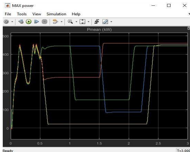
Fig.4.11: Maximum power output
