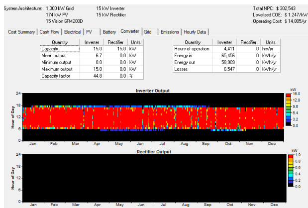
Fig. 4.6 Inverter output
