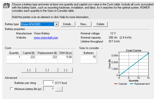
Fig. 3.2: Storage battery
