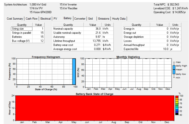
Fig. 4.7 Battery bank state of charge
