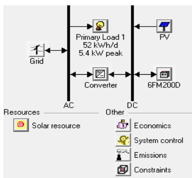
Fig 3.5 Model system
