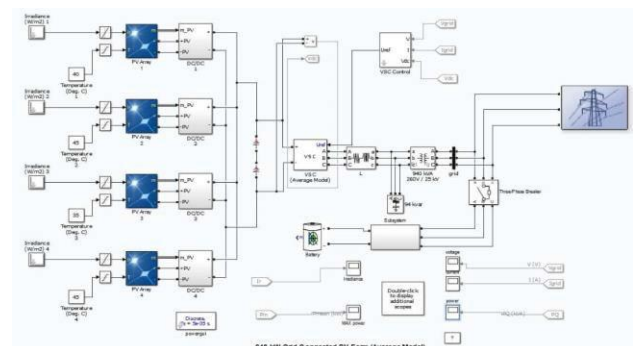
Fig.4.8: 940 kW Grid connected PV farm
