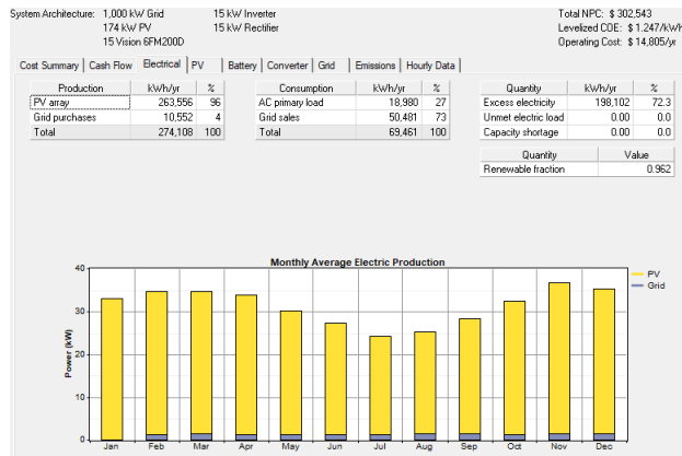
Fig.4.4: Monthly average electricity production.
