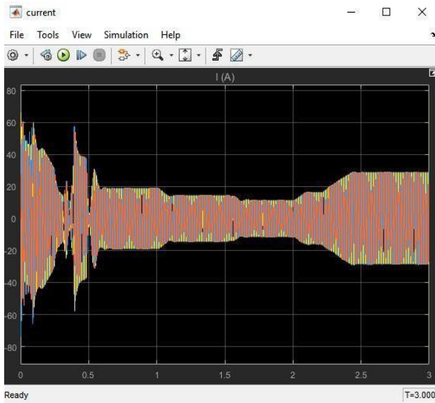
Fig. 4.9: Current output
