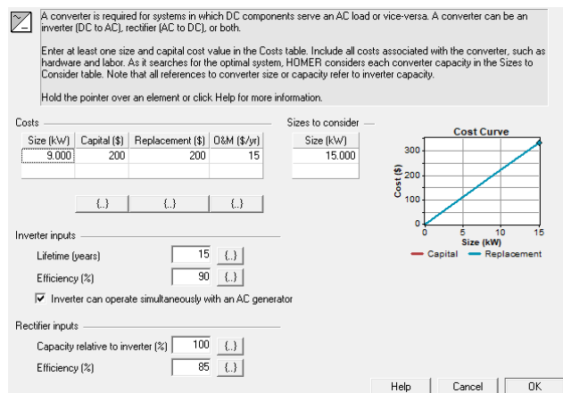
Fig.3.3 Inverter
