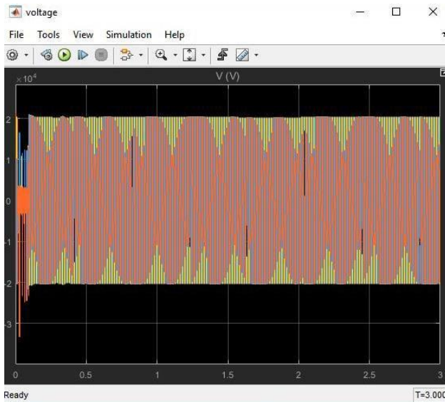
Fig.4.10: Voltage output
